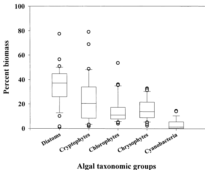
Fig. 4. Box plots of percent biomass in major algal divisions from 31 rivers in Ontario and western Quebec during summer base flows. The central line of each box is the median, the outer edges of each box are the 25th and 75th percentiles, and the limits of error bars are at the 10th and 90th percentiles.
