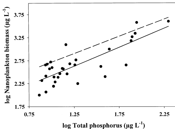
Fig. 2. Relationship between ambient total phosphorus concentrations and volume-converted nanoplankton (2–20- \mu\text{m} size class) biomass in 31 rivers of Ontario and western Quebec ( \log[\text{nanoplankton biomass}] = 0.82 \log \text{TP} + 1.61 ; r^2 = 0.63 , p < 0.001 , F_{1,29} = 49.3 ). The dotted line corresponds to the regression model relating total potamoplankton biomass to TP concentration ( \log[\text{potamoplankton biomass}] = 0.74 \log \text{TP} + 1.97 ; r^2 = 0.57 , p < 0.001 , F_{1,29} = 38.7 ).
