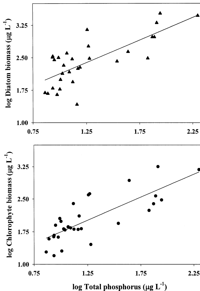
Fig. 5. (A) Relationship between ambient total phosphorus concentrations and diatom biomass ( \log[\text{diatom biomass}] = 1.09 \log \text{TP} + 1.04 ; r^2 = 0.57 , p < 0.001 , F_{1,28} = 36.7 ). (B) Relationship between ambient total phosphorus concentrations and chlorophyte biomass ( \log[\text{chlorophyte biomass}] = 1.06 \log \text{TP} + 0.69 ; r^2 = 0.62 , p < 0.001 , F_{1,28} = 45.8 ).
