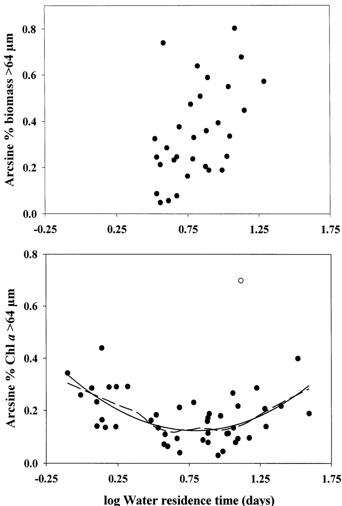
Fig. 3. Relationship between water residence time and the proportion of netplankton biomass (>64 \mu\text{m} ) measured as (A) volume-converted biomass and (B) Chl a . For the Chl a data, a locally weighted sequential smoothing technique (LOWESS) provided a model-free assessment of the nonlinear trend (dotted line), which was subsequently approximated with a quadratic model (solid line: \arcsin[\% \text{Chl } a (>64 \mu\text{m})] = 0.29 - 0.42 \log \text{WRT} + 0.27(\log \text{WRT})^2 ; r^2 = 0.37 , p < 0.001 , F_{2,42} = 12.4 , n = 45 rivers). One outlier (open circle) was removed from the Chl a model.
