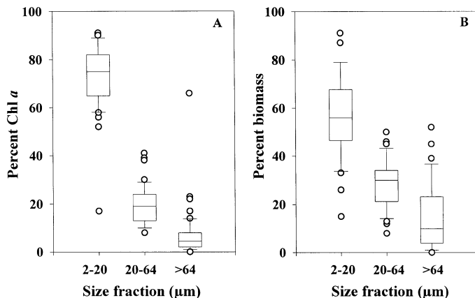
Fig. 1. Proportion of potamoplankton Chl a and biomass in three size fractions (2–20, 20–64, and >64 \mu\text{m} ). Box plots represent (A) the distribution of percent Chl a ( n = 46 ) and (B) percent biomass ( n = 31 ) among rivers for each fraction. The central line of each box is the median, the outer edges of each box are the 25th and 75th percentiles, and the limits of error bars are at the 10th and 90th percentiles.
